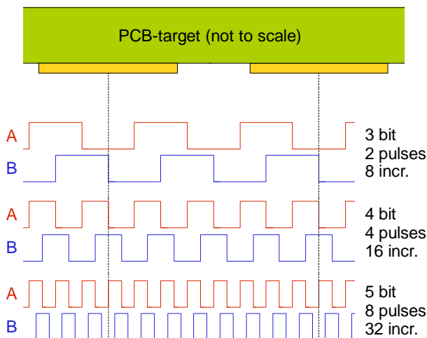
Fig. 1 A quad B signals over one period of 1.2 mm with interpolation 3 – 5 bit.
